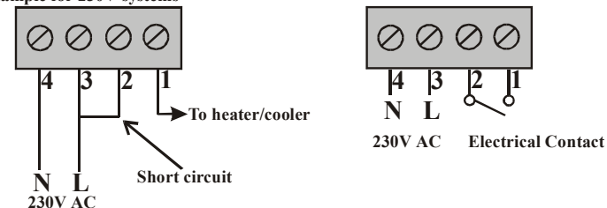
Wiring diagram
